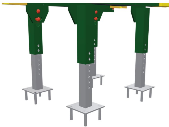
— Patas regulables
